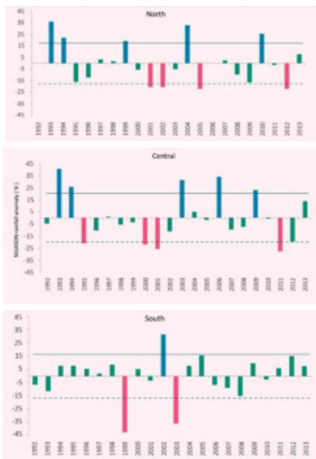
Figure 4-4: Flood and drought years for: (a) northern, (b) central and (c) southern Maldives based on Maldives monsoon rainfall. Cross bars indicate the flood years, dotted bars indicate the drought years. Solid line is the sum of mean and standard deviation and dotted line is the difference between mean and standard deviation.
